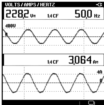
Figure 5. VOLTS/AMPS/HERTZ screen
